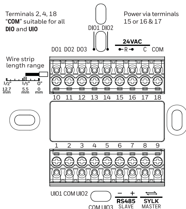
Fig. 1. Terminals of TC300 Thermostat
